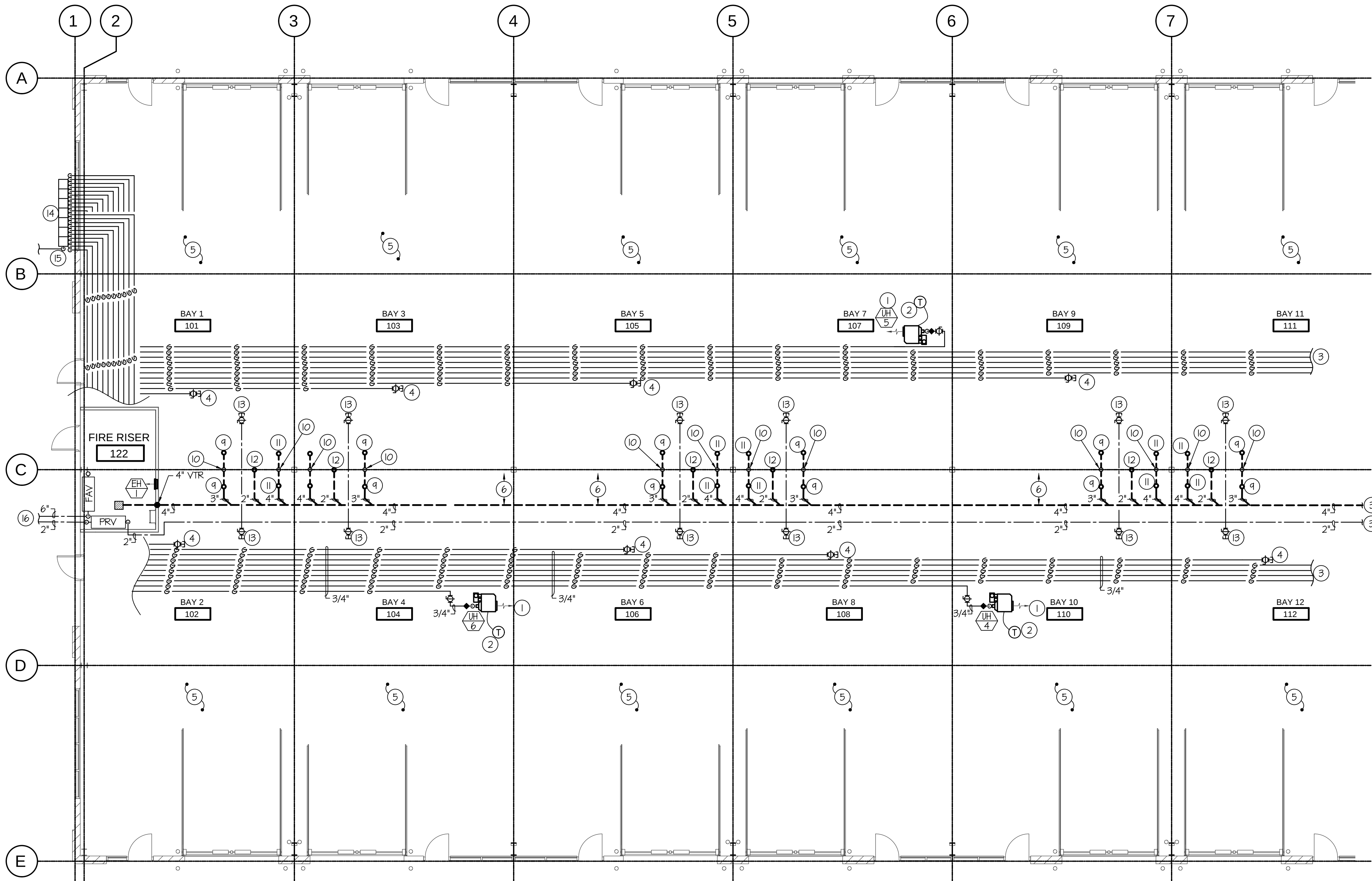
MECHANICAL & PLUMBING "A" FLOOR PLAN SCALE: 1/8" = 1'-0"
